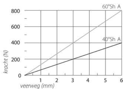
Belasting F_z
